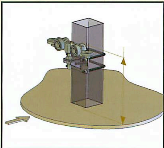
SUPPORT RAIL WHEEL ASSEMBLY
